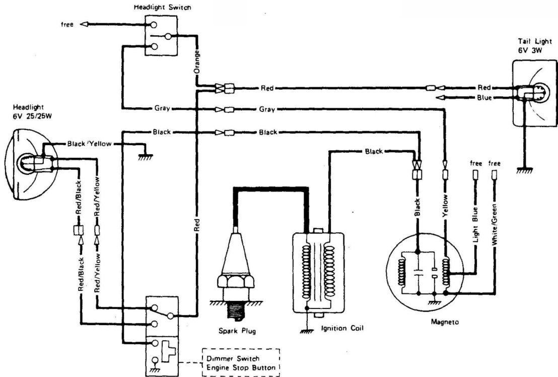
KV75 Wiring Diagram
