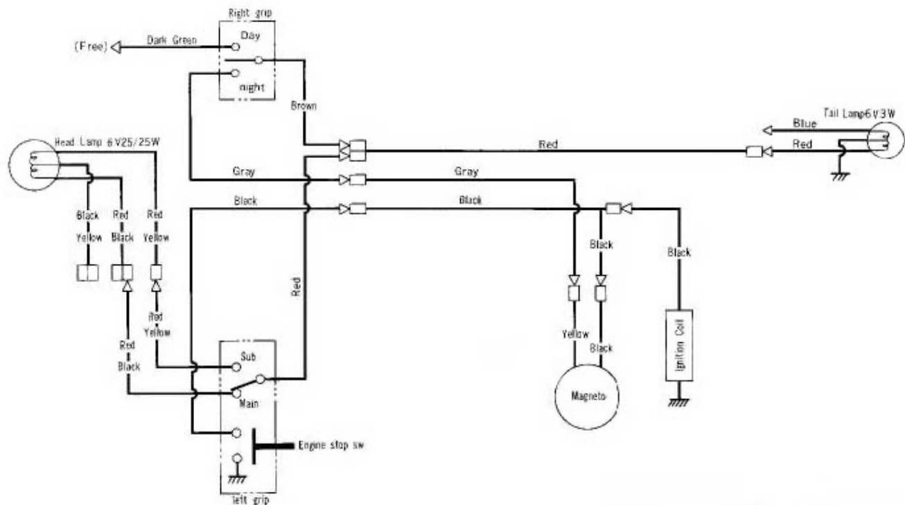
MT-1 Wiring Diagram
